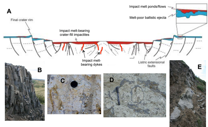
Fig. 1A. Schematic cross section of a typical complex impact crater showing the distribution of impact melt-bearing impactites. B. Volatile-free/poor impact melt rocks from the ejecta of the Mistastin Lake impact structure, Canada. C and D. Volatile-rich impact melt-bearing breccias from the Ries impact structure, Germany (D) and the Mistastin structure (D). The sub-vertical orange features at the left of C are degassing pipes. E. Volatile-rich impact melt-bearing breccia dyke intruded into the crater floor at the Mistastin structure.
